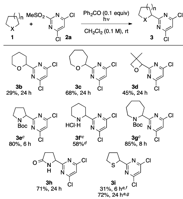
Scheme 3. Coupling between Saturated Heterocycles and 4,6-Dichloro-2-methanesulfonylpyrimidine a,b
