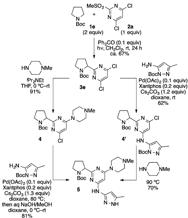
Scheme 4. Preparation of an Analogue of the Aurora Kinase Inhibitor, MK-0457
